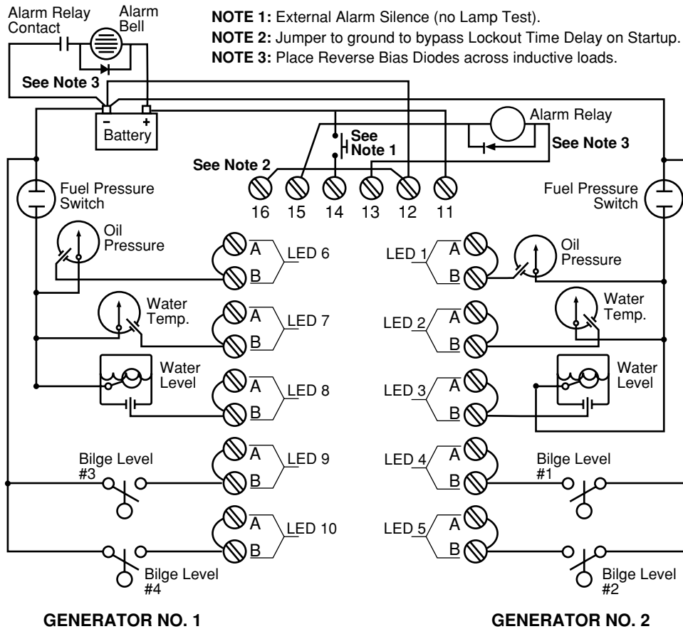
Figure 3: ST10AS Typical Circuit Diagram
