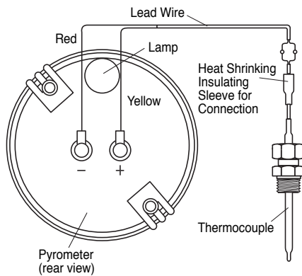
10705147 (00-00-0956) Single Port
