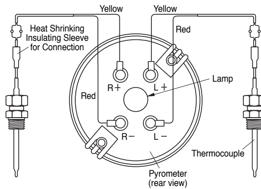
10705146 (00-00-0819) Dual Port
